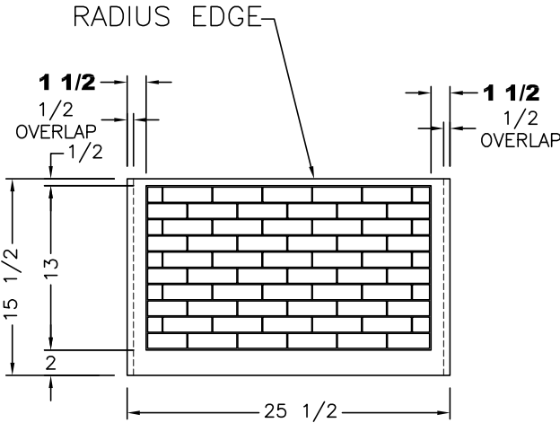
VIEW B
