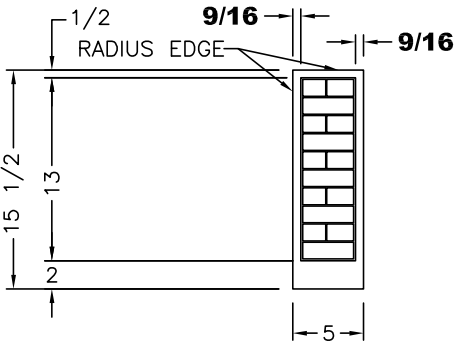
VIEW A
