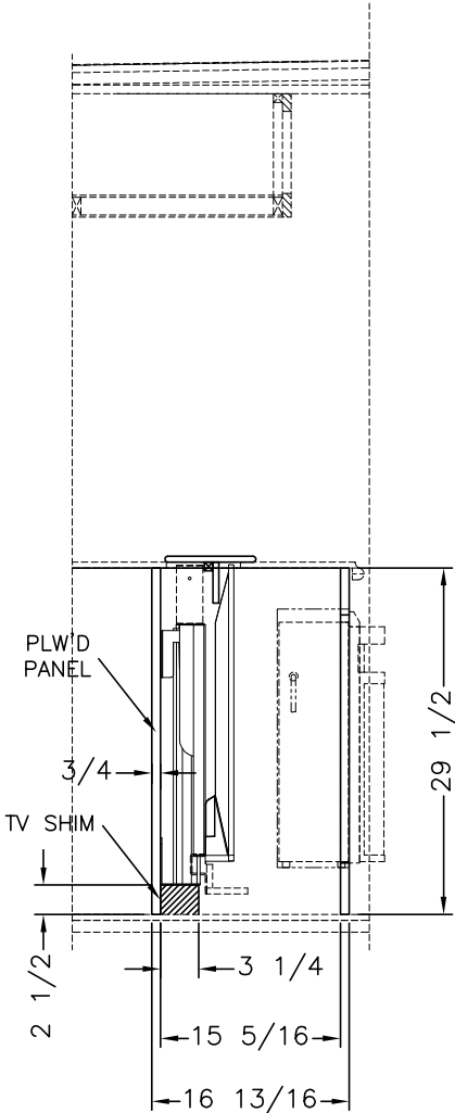
SIDE SECTION (A)
