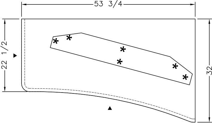
1/2" SOLID SURFACE CABINET TOP ▶ - DENOTES A FINISHED EDGE * - PENCIL EDGE
