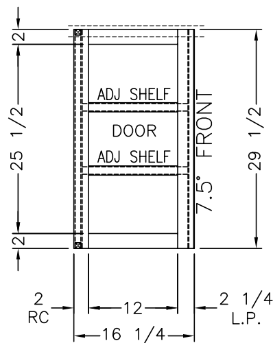
FRONT VIEW (A) (1) 12 3/8x26 DOOR
