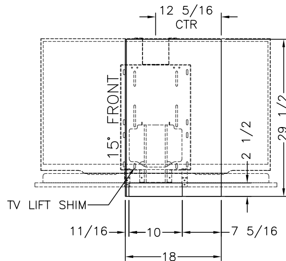
FRONT VIEW 3/4" MOUNTING PANEL
