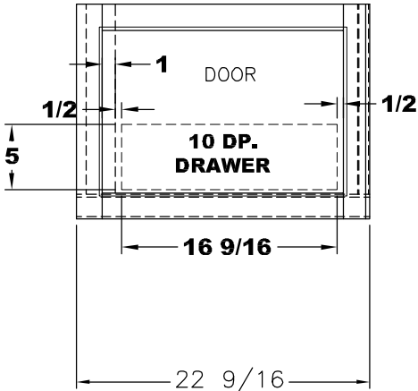
VIEW (H)
