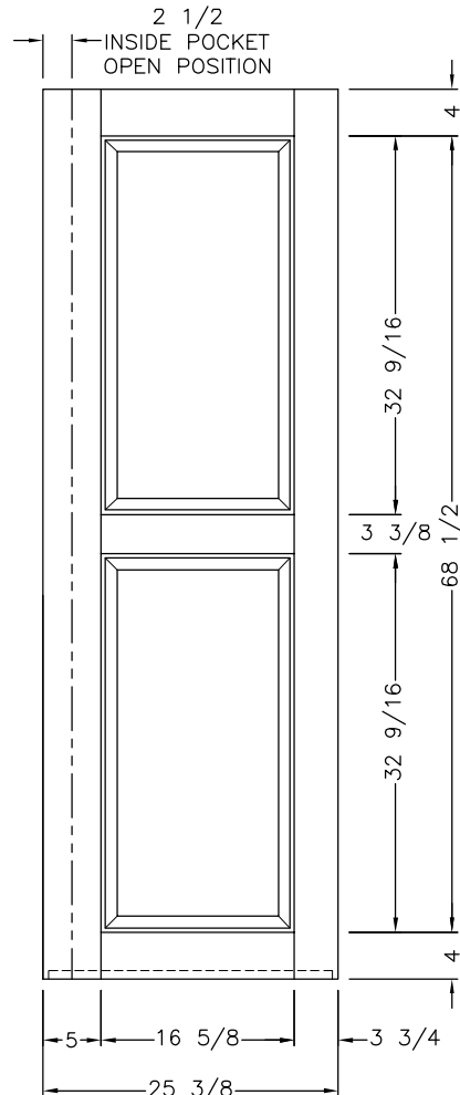
BEDROOM SIDE
