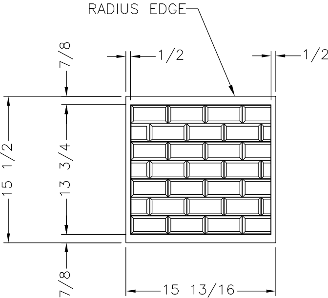
VIEW A
