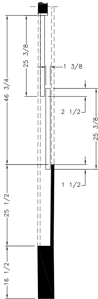
PLAN VIEW
