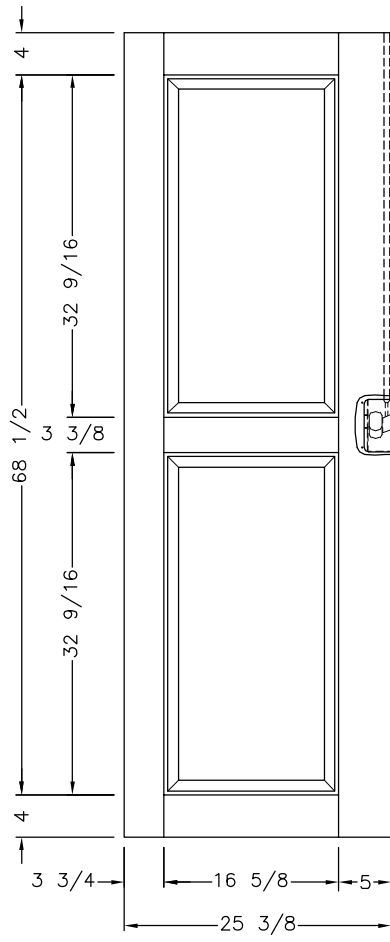
KITCHEN SIDE
