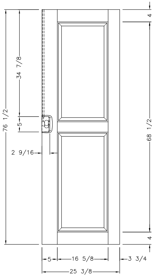
BEDROOM SIDE
