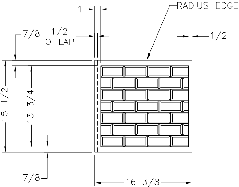
VIEW B
