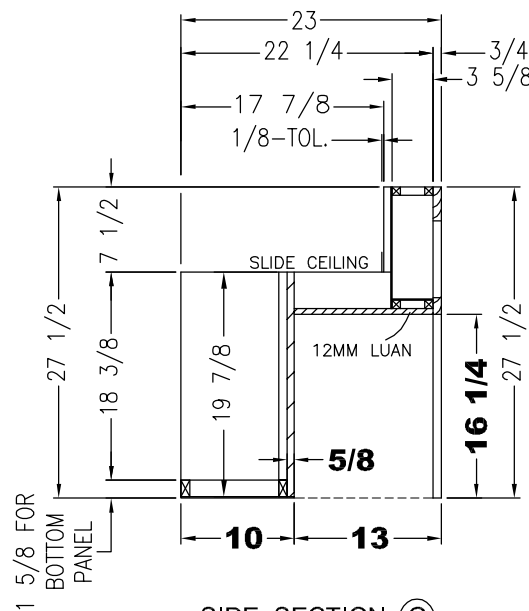
SIDE SECTION (G)
