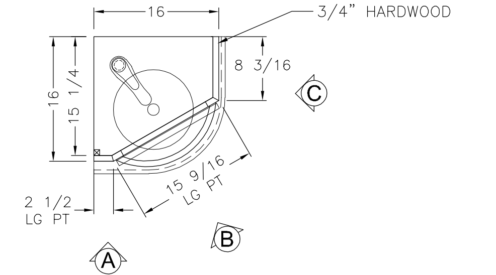
LAV. BASE (TOP VIEW)
