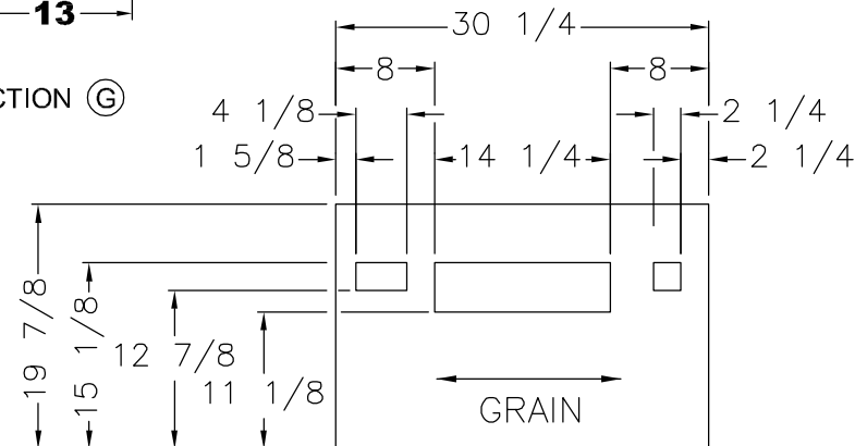
5/8 PLYWOOD DETAIL
