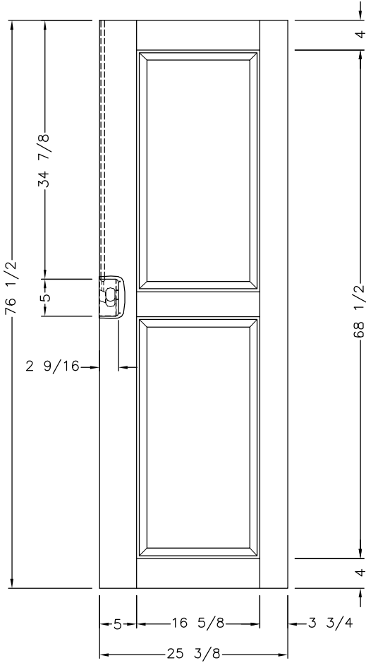
BEDROOM SIDE
