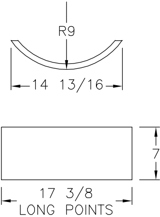
FRONT COVER LAID OUT FLAT
