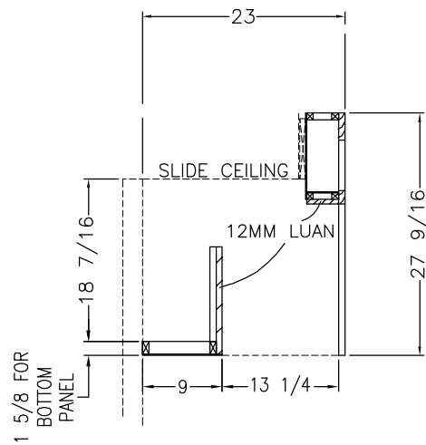
SIDE SECTION J
