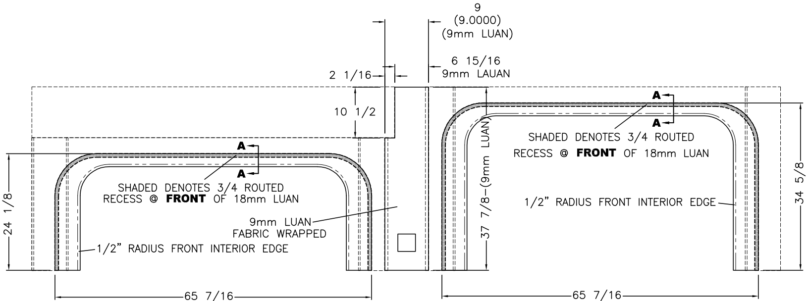
FRONT VIEW 9mm/18mm LUAN FABRIC WRAPPED
