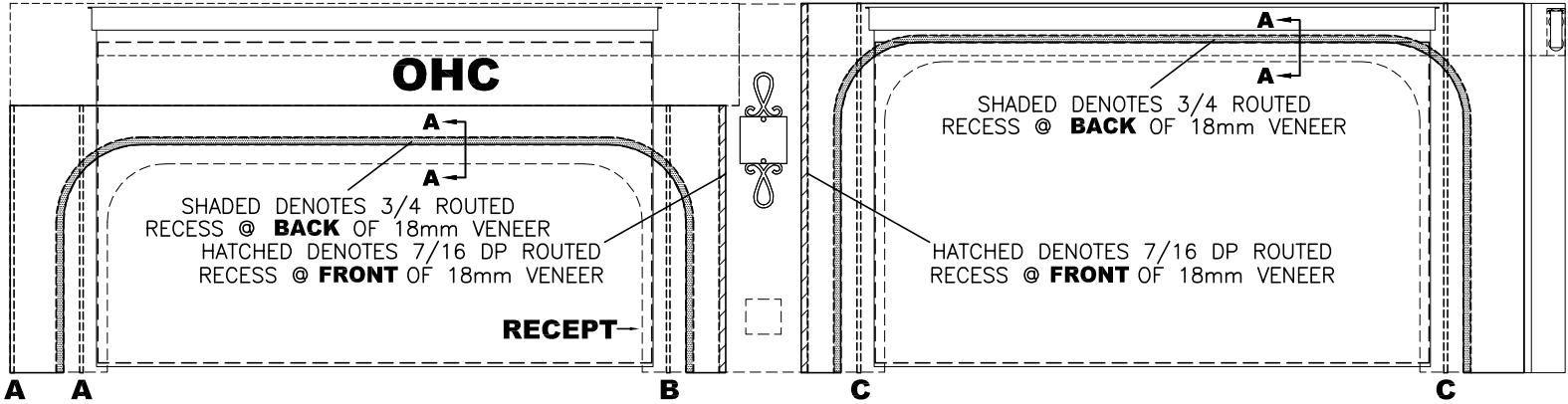
FRONT VIEW 18mm VENEER MAIN PANELS
