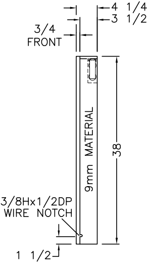
LEG-C (2-REQ'D)
