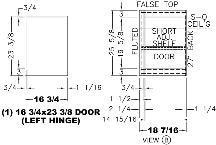
VIEW (B)
