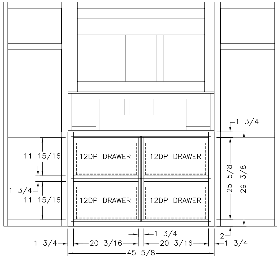
FRONT
