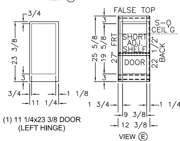
VIEW (E)
