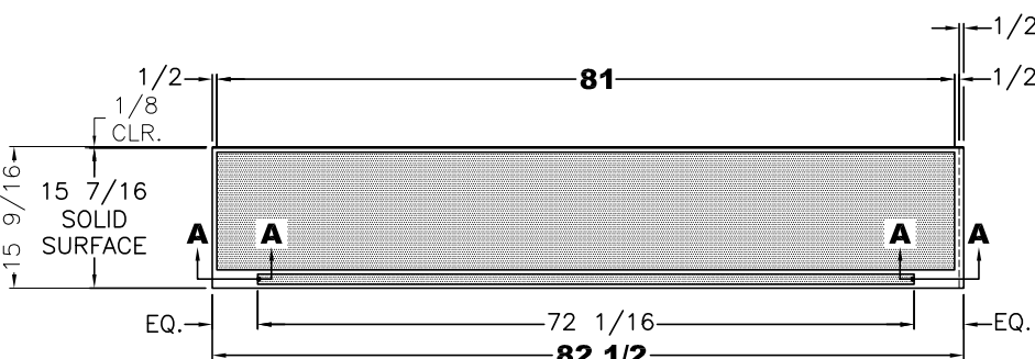
SHADE DENOTES 3/8" RECESS FOR TILE INLAY
