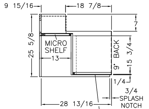
VIEW (K)
