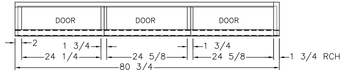
FRONT VIEW
