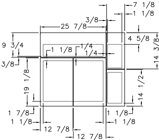
VIEW B OVERLAPS
