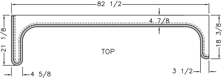
CNC NOTE: SHADED EDGE DENOTES 1/4" DP RECESS
