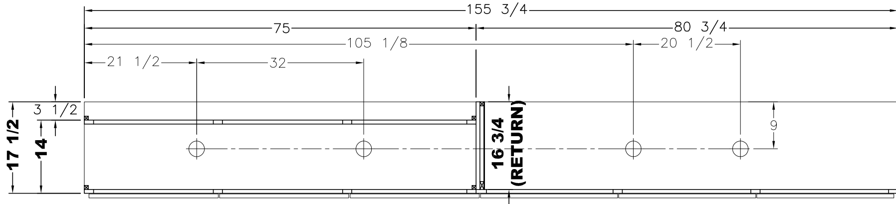
PLAN VIEW
