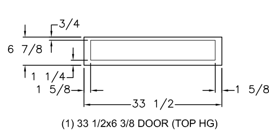
VIEW (C)
