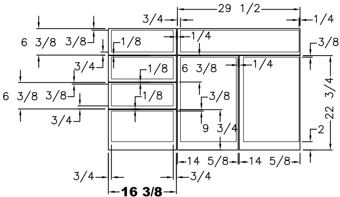
VIEW A OVERLAPS
