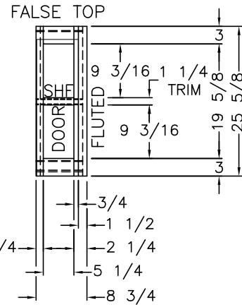
VIEW (G)
