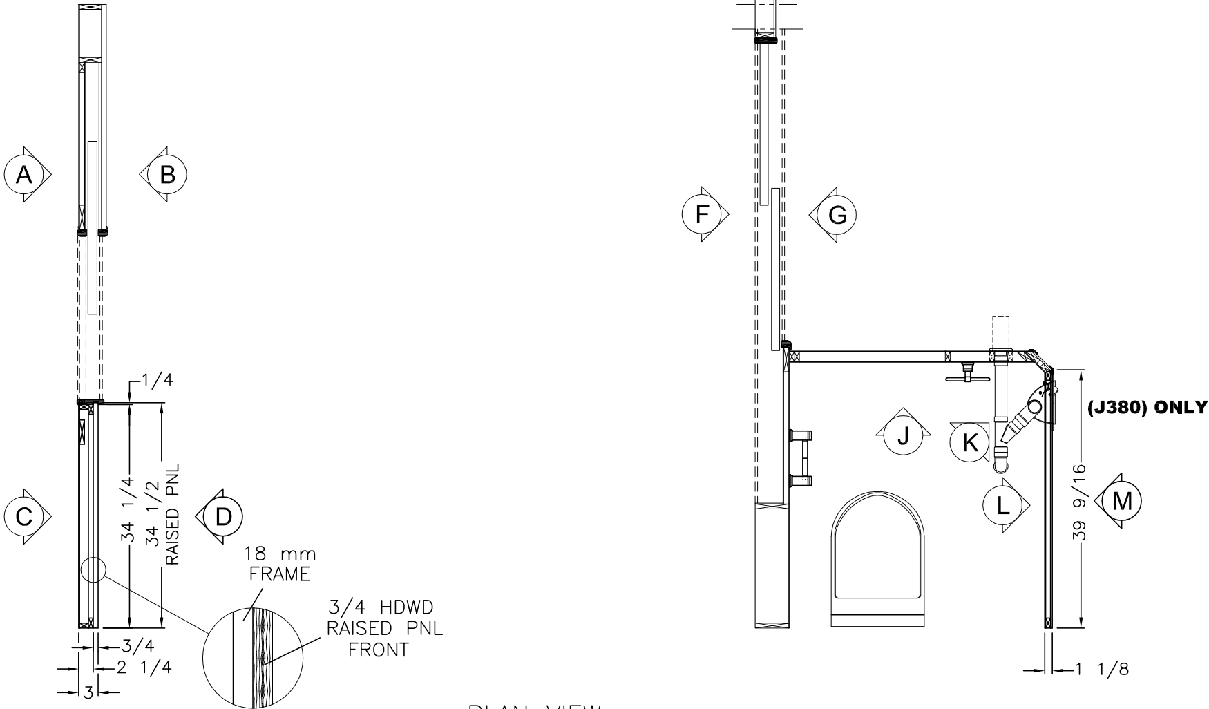
PLAN VIEW
