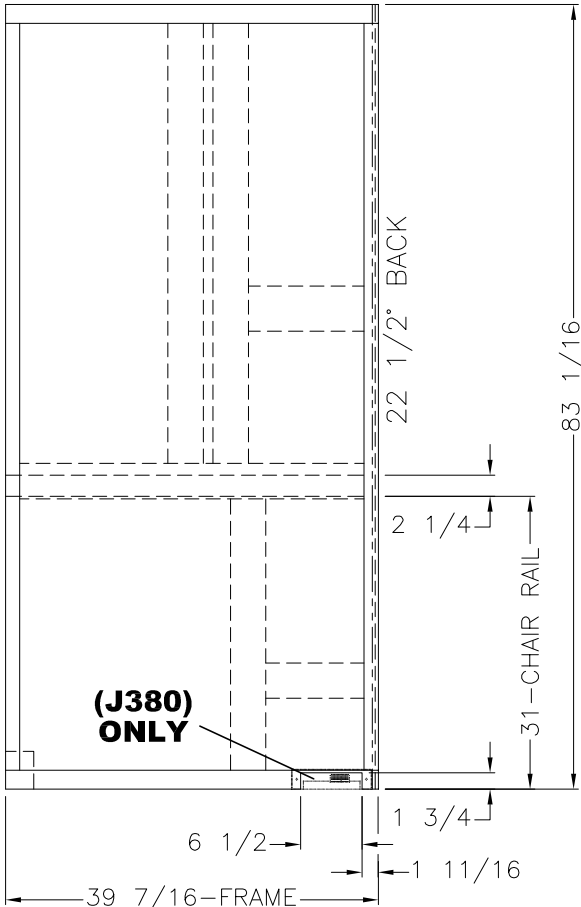
VIEW (M) FRAME
