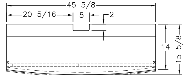
SOLID SURFACE TOP
