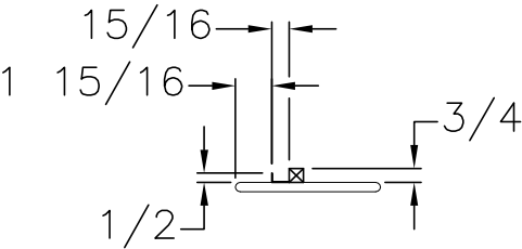
END VIEW/BOTTOM UP
