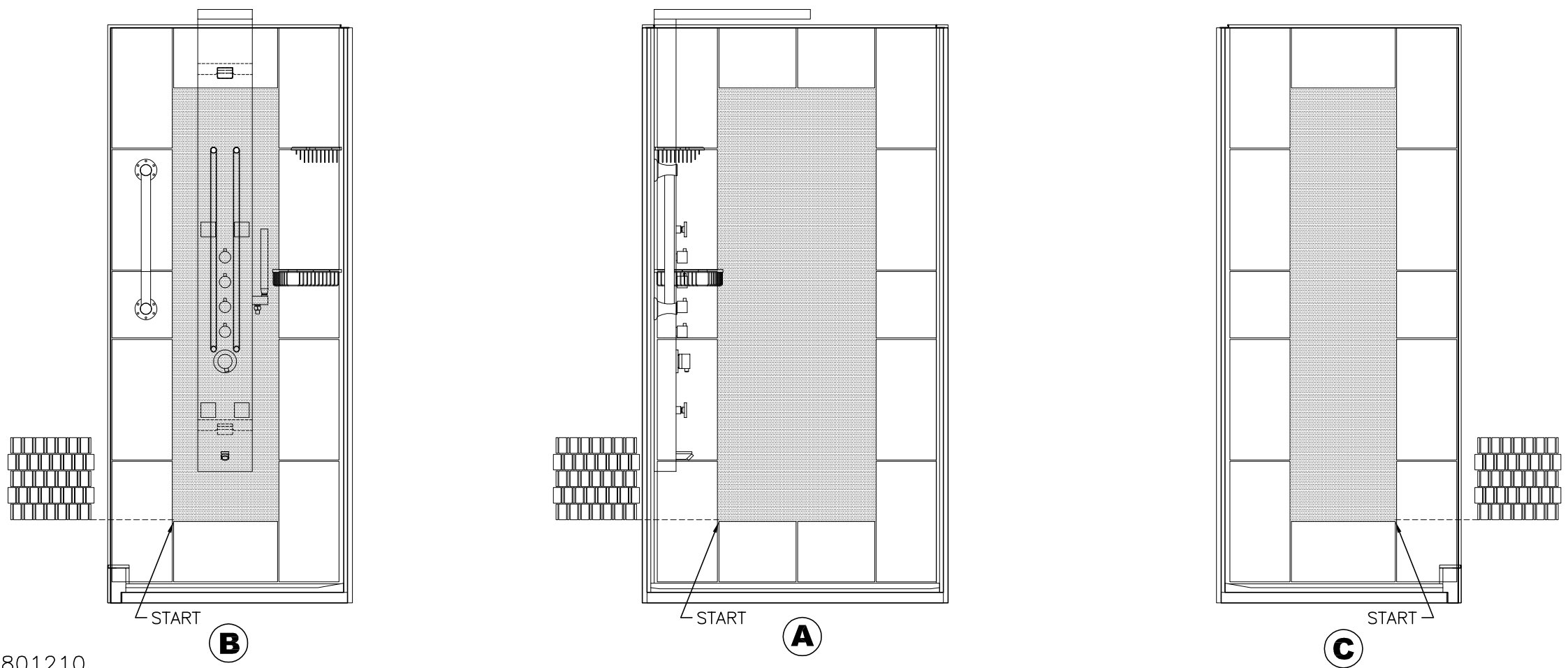
PLYW'D/FOAM WALLS/TILE LAYOUT
