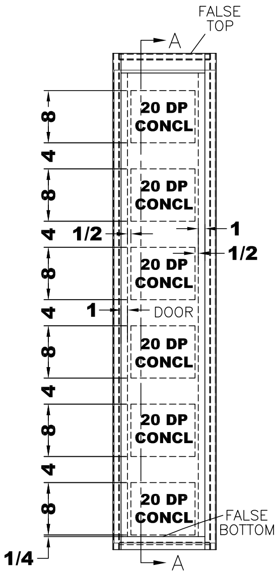
FRONT VIEW
