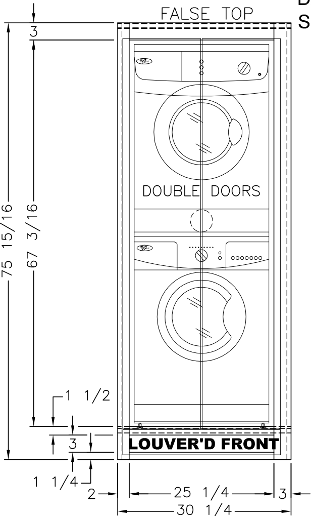
FRONT VIEW (2) 13 5/8x67 7/8 LOUVERED DOORS (1) 4 3/8x27 1/2 LOUVERED FRONT
