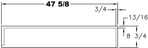
FALSE FRONT O'LAPS
