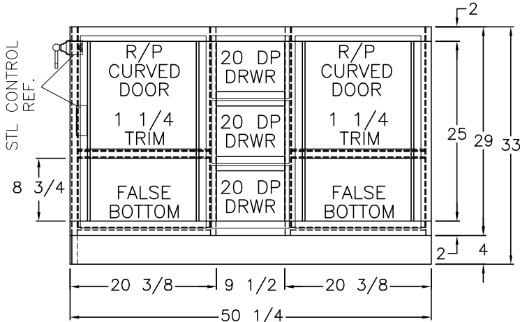
FRONT VIEW (3) 8 3/4x10 3/4 DRAWER FRONTS (2) CURVED DOORS
