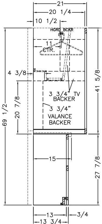
SECTION (A) PLAN/DRESSER FRONT/SECTION
