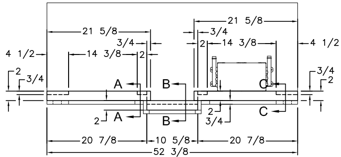
PLAN VIEW (STILED TOE-KICK)
