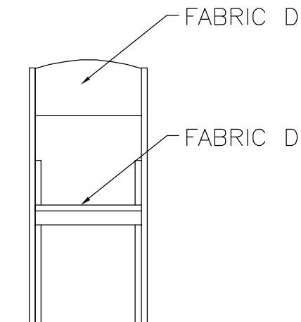
FOLDING CHAIR
