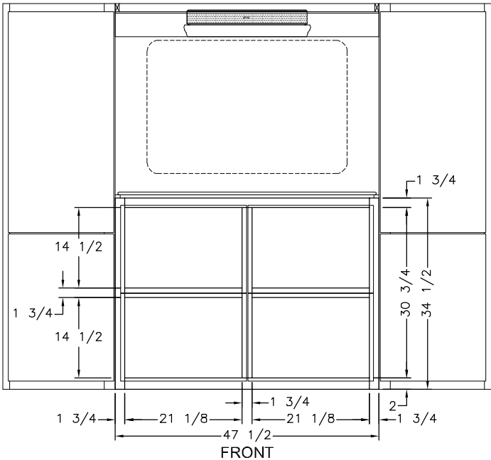
(4) 15 3/4x22 5/8 FALSE DRAWER FRONTS
