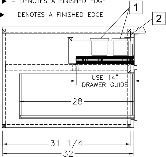
SIDE SECTION A
