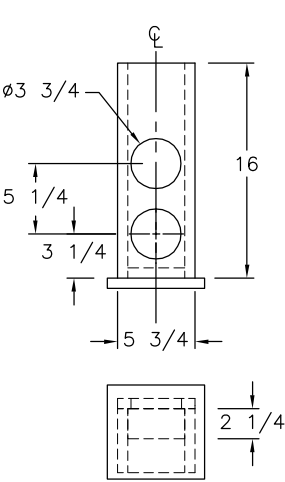
TOP DRAWER DETAIL VIEW
