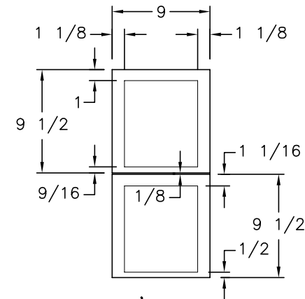
(2) 9 1/2x9 FRONTS
