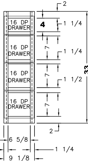
(1) 5 3/8x8 7/8 DRAWER FRONT (3) 8x8 7/8 DRAWER FRONTS
