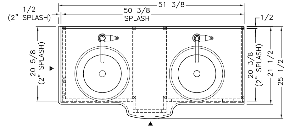
1/2" SOLID SURFACE ▲ – DENOTES A FINISHED EDGE
