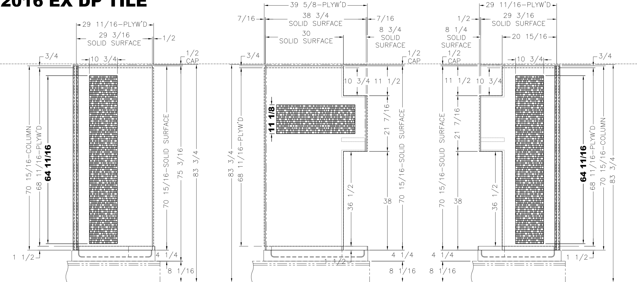
VIEW A
