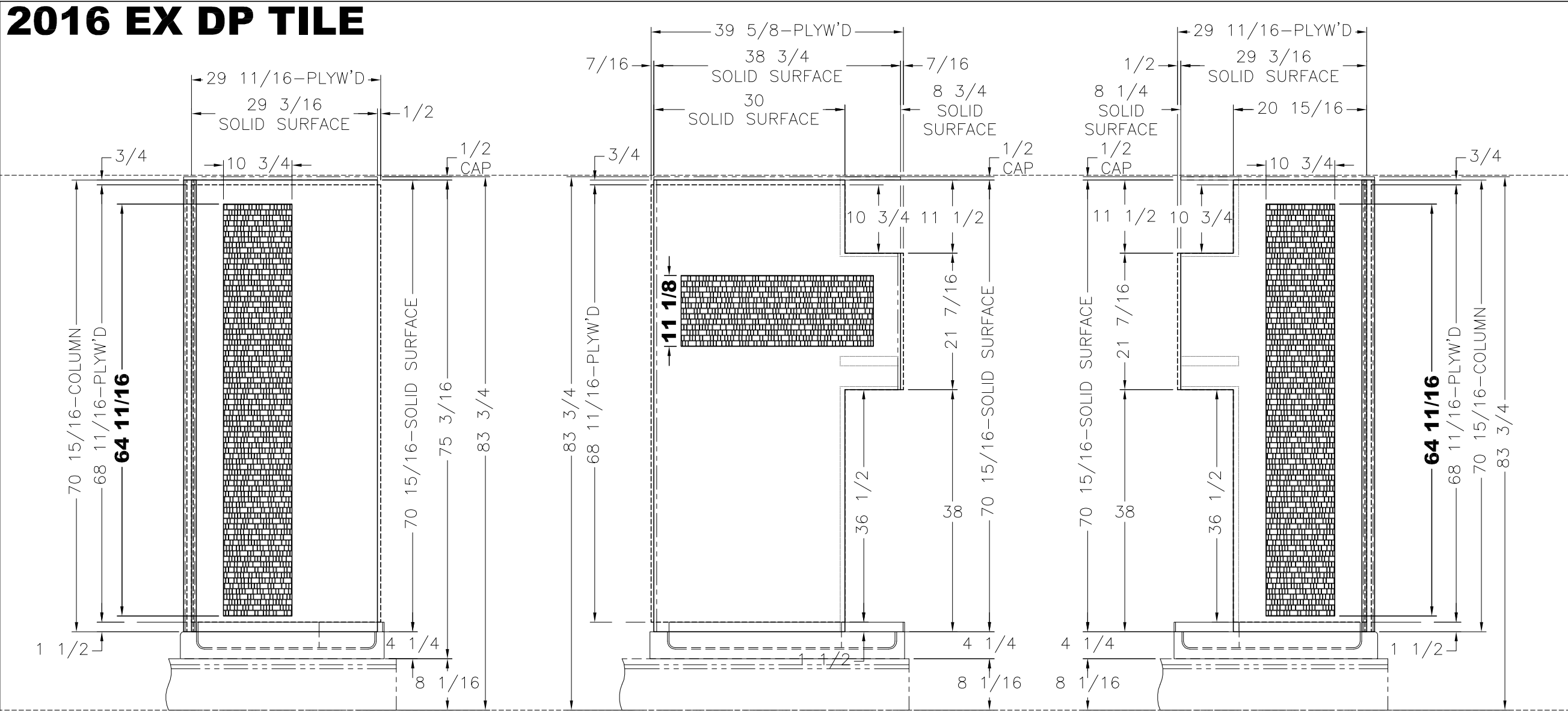
VIEW A
