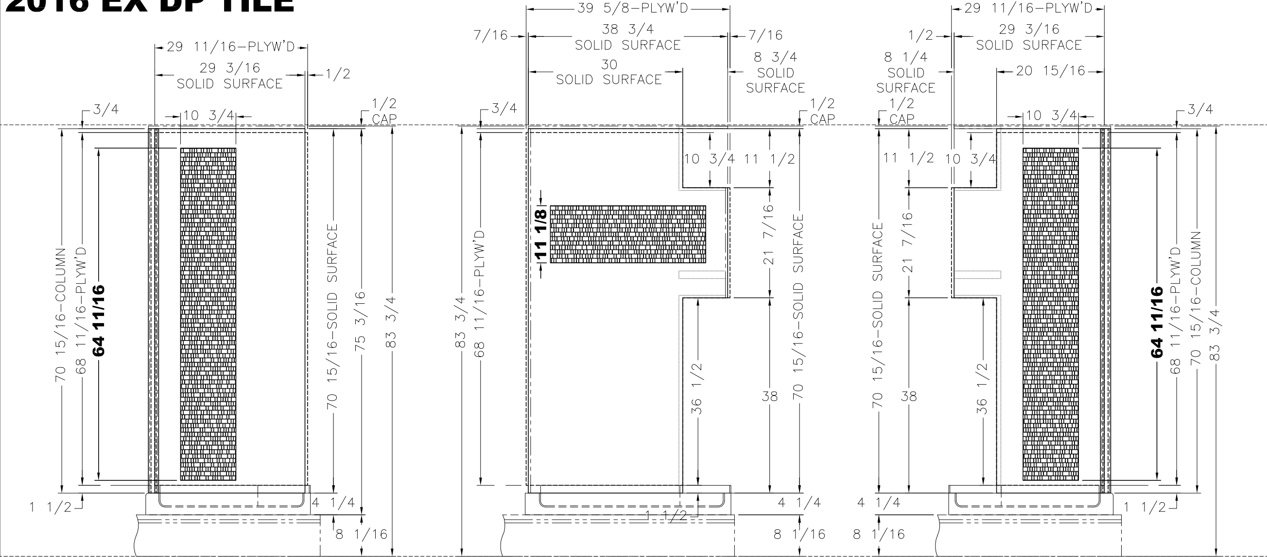
VIEW A
