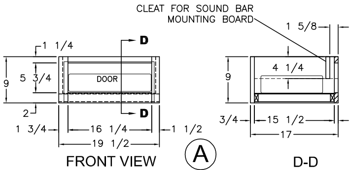
(1) 7 7/8 x17 1/2 DOOR (TOP HG)
