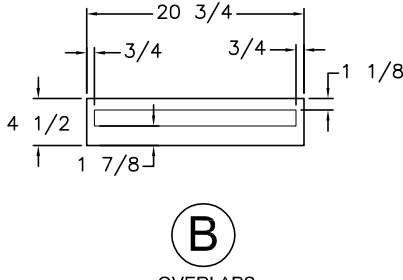
(1) 4 1/2x20 3/4 FALSE FRONT
