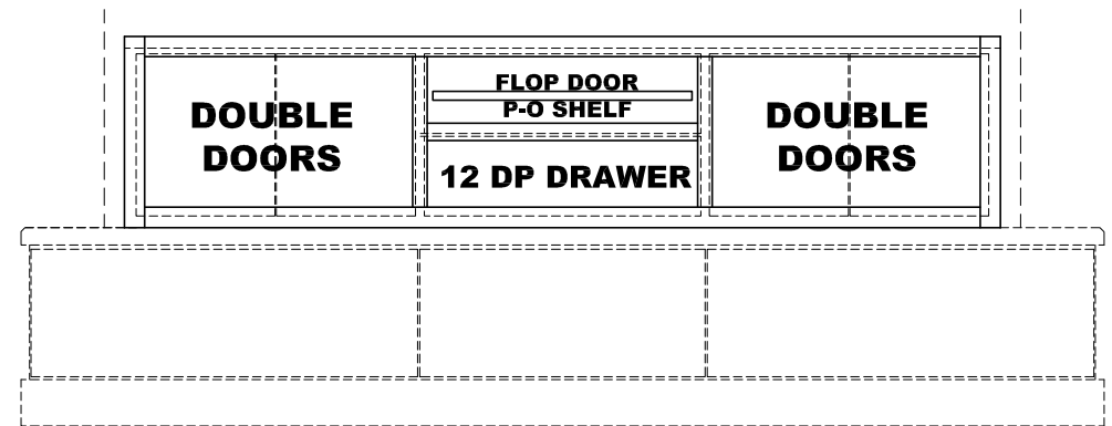
FRONT VIEW (UPPER SECTION) (2) 6 7/8x23 7/8 DRAWER FRONTS (4) 12x14 DOORS
