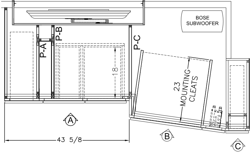
PLAN VIEW OPT (J528)
