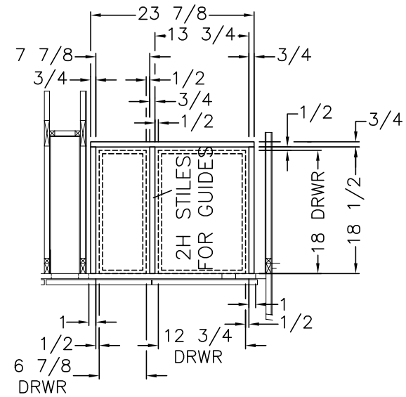
VIEW A DRAWER DETAIL
