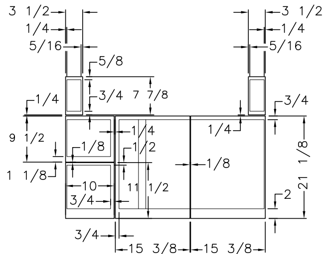
VIEW A OVERLAPS
