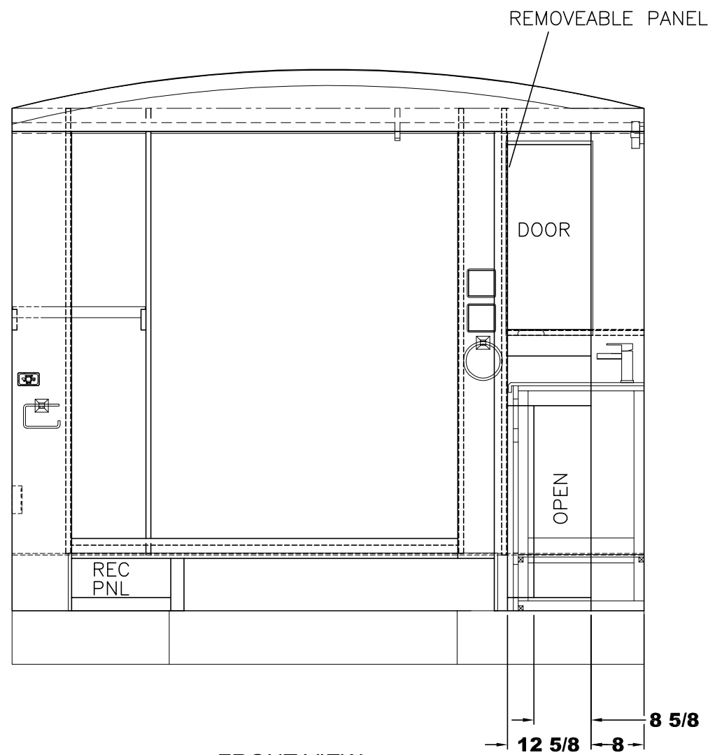
FRONT VIEW (1) 13 1/8 X 29 3/8 FALSE DOOR ON CATCHES W/ROUTED FINGER PULL BOTTOM EDGE
