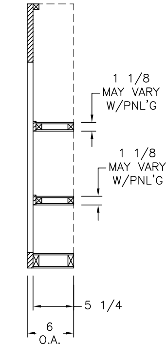
SIDE SECTION (A)
