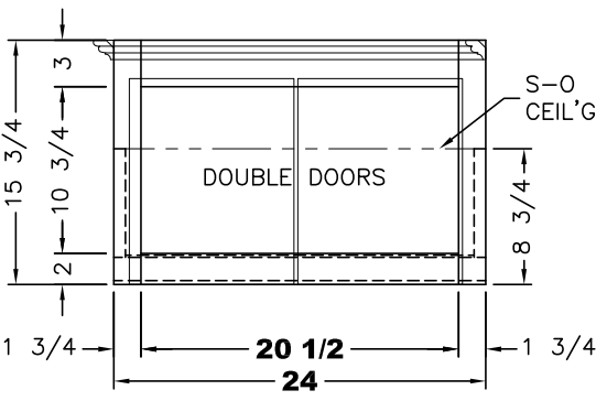
(2) 10 5/8 X 13 1/4 DOORS
