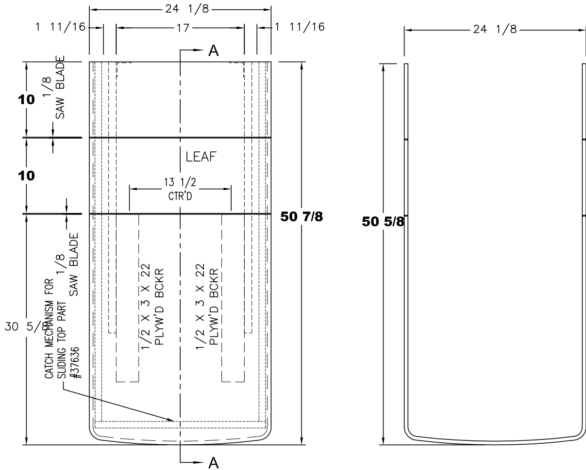
SLIDING TOP COUNTERTOP AND EDGE TREATMENT
