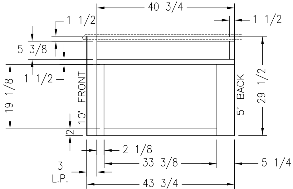
VIEW A
