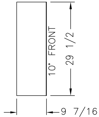
VIEW C
