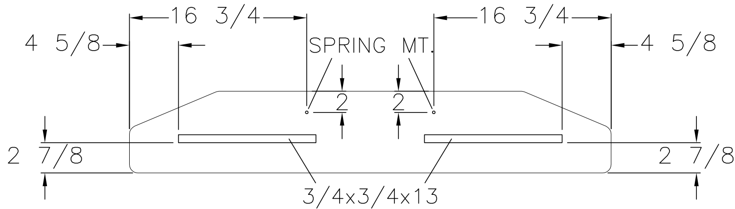
BOTTOM VIEW
