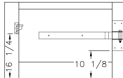
FIREPLACE HARDWARE
