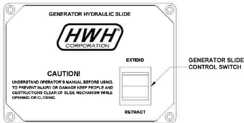
GENERATOR SLIDE OPERATOR'S PANEL
