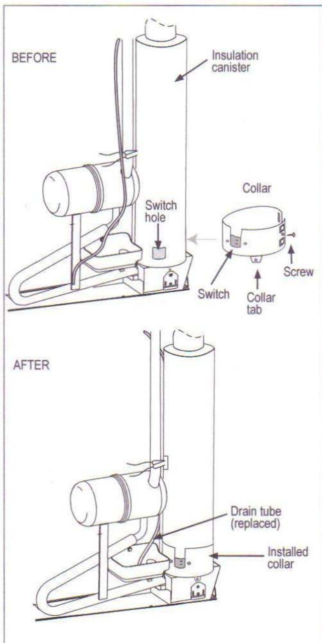
Figure 5. Installing the Metal Collar and Switch
