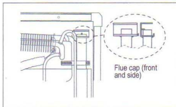
Figure 8. Protecting the Flue Cap
